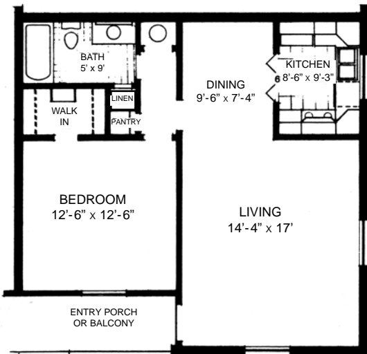
ONE BEDROOM ONE BATH - 24 UNITS BUILDINGS C, D, & G 719 sq. ft.
