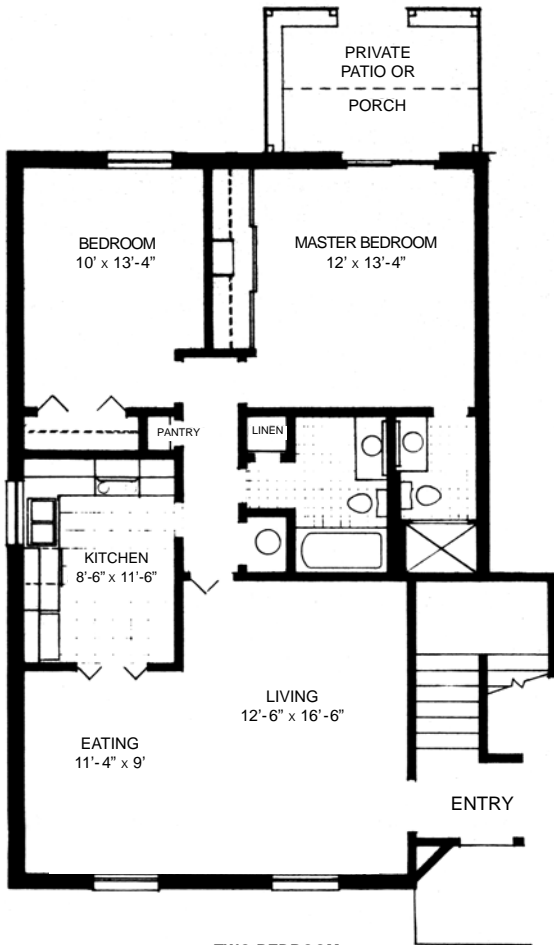
TWO BEDROOM TWO BATH - 22 UNITS BUILDINGS A, B, & J 1072 sq. ft.
